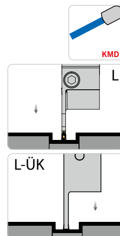
Left basic holder and left monoblock holder shown Adattatore base sinistro e stelo monoblocco sinistra in figura Support gauche et outils monobloc gauche montés
