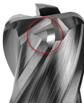
Normal end-mill
